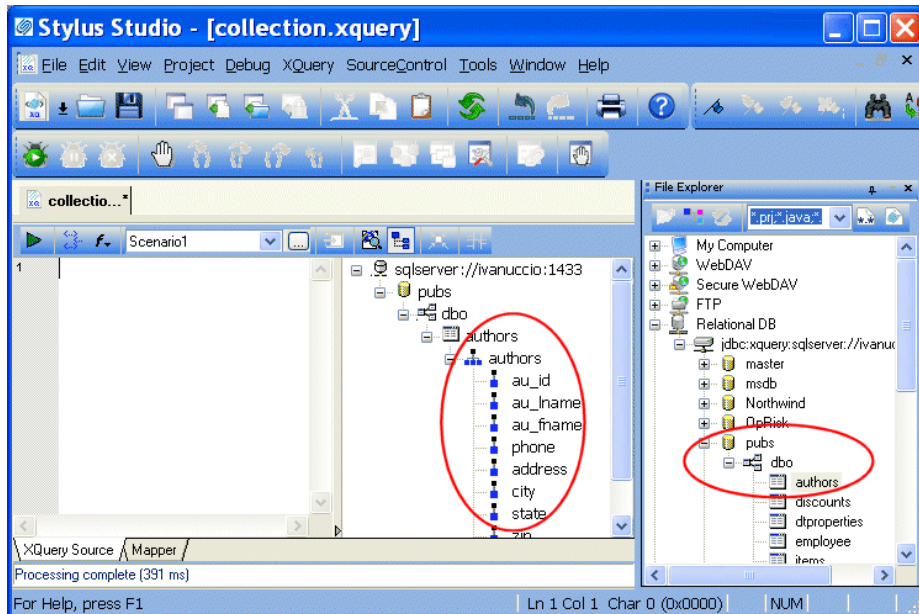
Figure 325. Schema Pane Shows Table and View Columns
