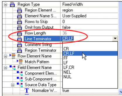
Figure 165. Manually Setting the Line Terminator Character
