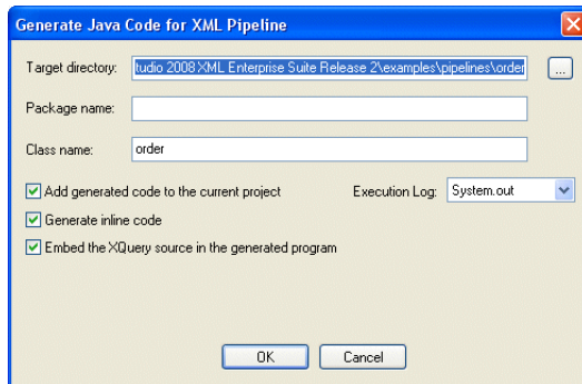
Figure 428. Generate Java Code for XML Pipeline Dialog Box
