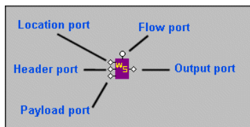
Figure 342. Port Types for the wscall Function block
