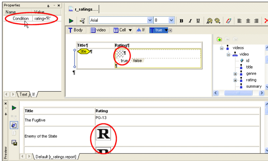
Figure 472. Example of an If Component
