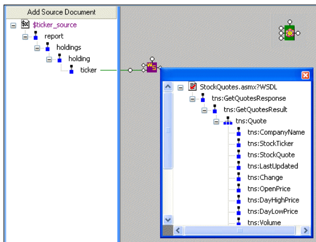
Figure 353. Selecting Output
