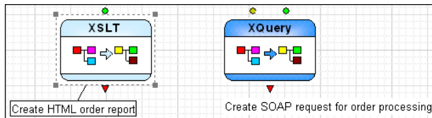
Figure 423. Pipeline Labels
