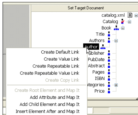
Figure 298. Linking Using the Right Mouse Button Displays a Shortcut Menu
