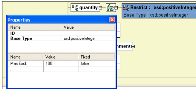
Figure 253. Properties Window with Restricted Type Facets
