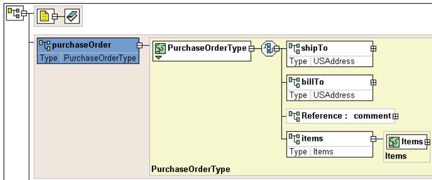
Figure 53. Background Colors Show Global and Local Types
