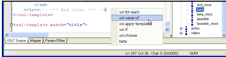
Figure 190. Stylus Studio Displays XSLT Instructions for Quick Editing
