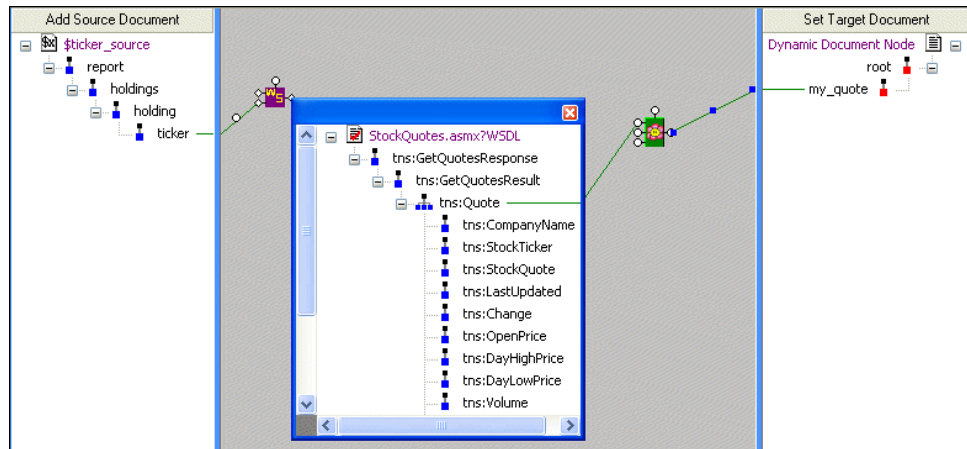
Figure 354. Mapping the Web Service to a FLWOR Block
