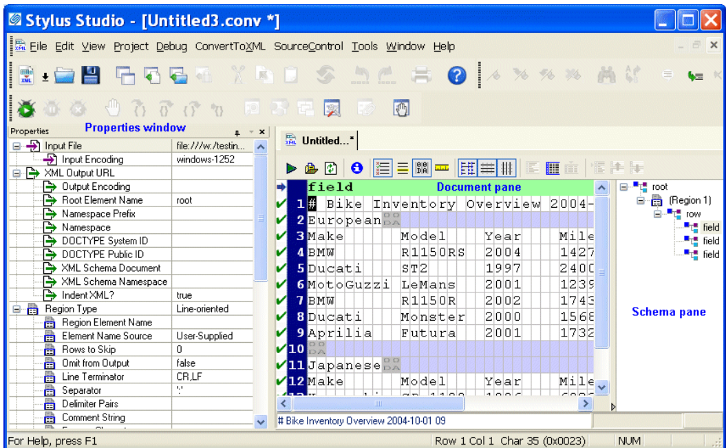
Figure 145. Custom XML Conversion Definition Editor
