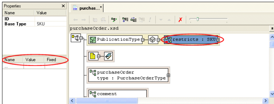
Figure 270. Facets for Describing Restrictions
