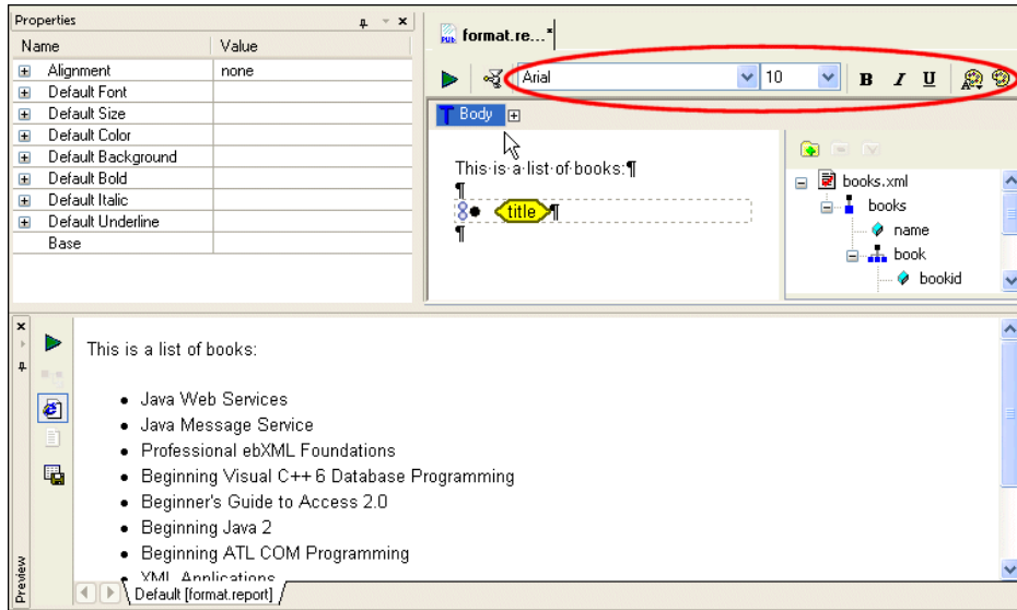
Figure 483. Default Format Settings
