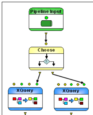
Figure 416. Choose Node in retrieveData.pipeline
