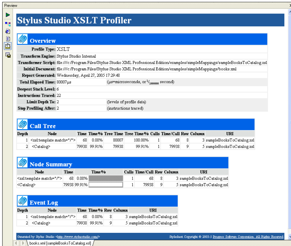
Figure 241. XSLT Profiler Report
