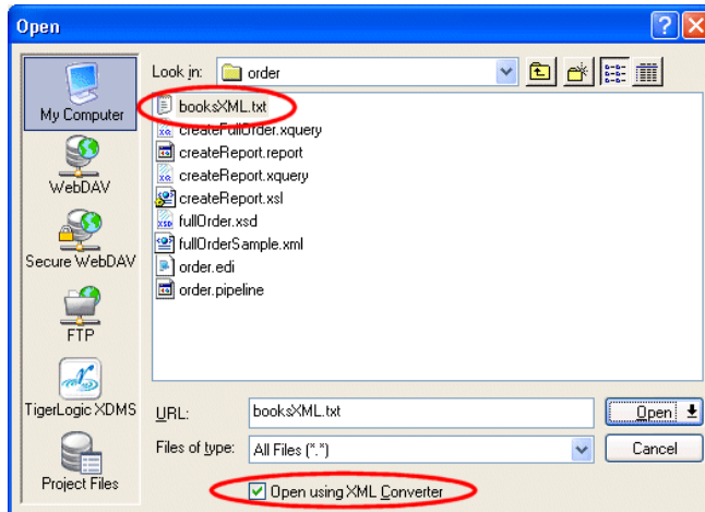
Figure 395. Using Non-XML Data as an XQuery Data Source
