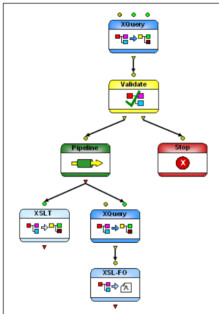
Figure 384. Diagram of getHoldings.pipeline
