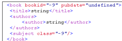
Figure 103. Complete XML Fragment Inserted Using Sense:X
