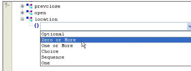
Figure 14. Drop-Down List for Modifier Values
