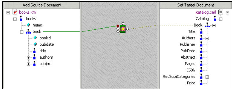
Figure 349. Mapping Typical Function Blocks in XQuery Mapper
