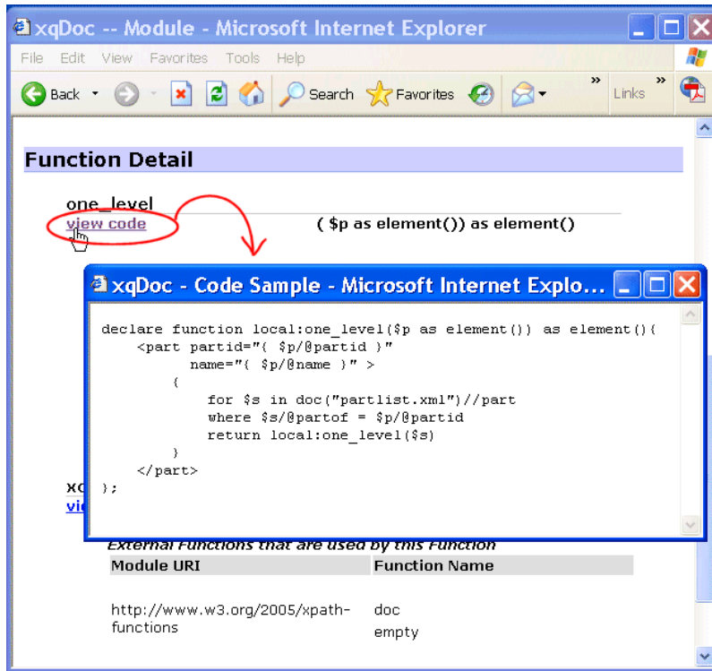
Figure 340. Viewing an XQuery Code Sample
