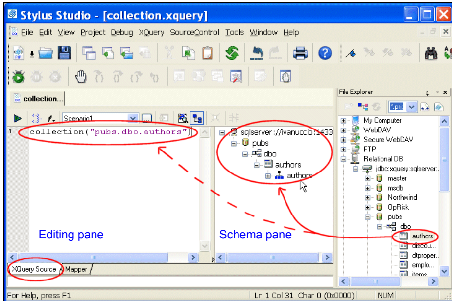
Figure 323. collection() Statements are Created Automatically
