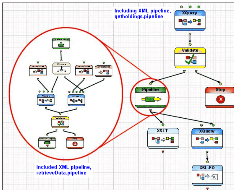
Figure 413. Illustration of an Included Pipeline ( retrieveData.pipeline )
