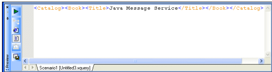
Figure 316. Predicate Result
