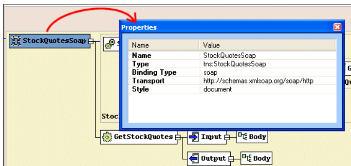
Figure 375. Properties Window
