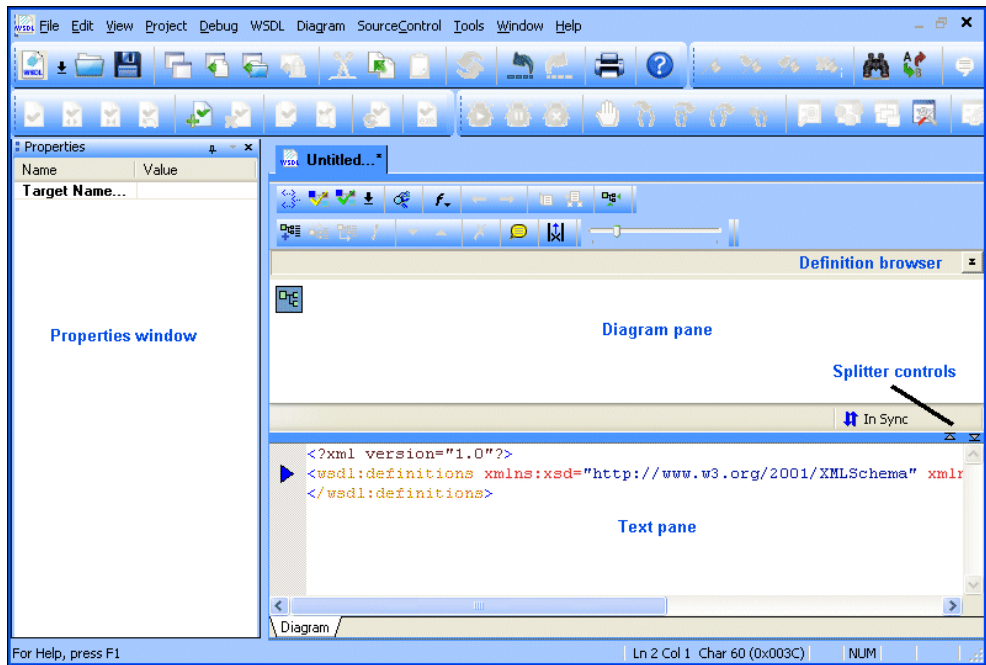
Figure 372. WSDL Editor
