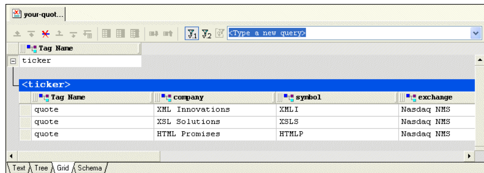
Figure 17. Grid Tab
