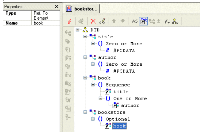
Figure 48. Finished bookstore.dtd
