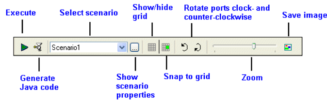
Figure 386. XML Pipeline Editor Toolbar Buttons
