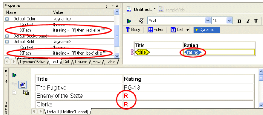
Figure 494. Finished Example Report
