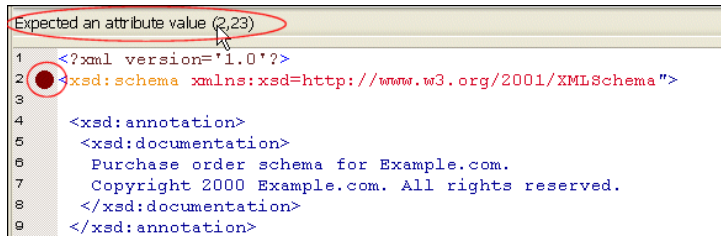
Figure 56. Text Pane Highlights XML Schema Errors
