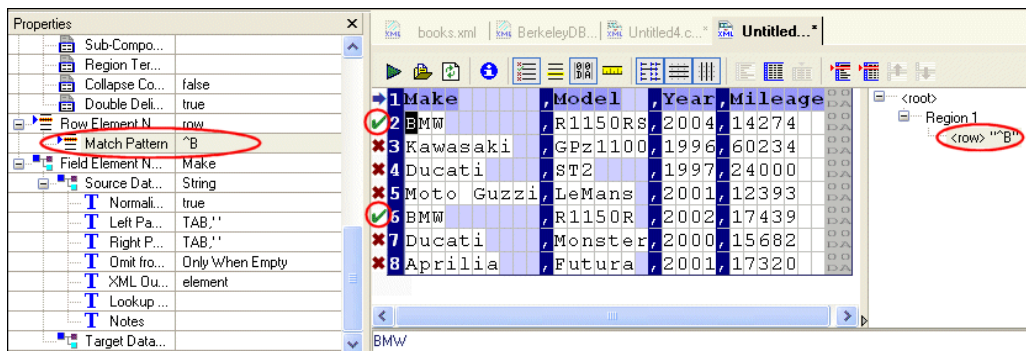
Figure 175. Match Pattern – Definition and Display
