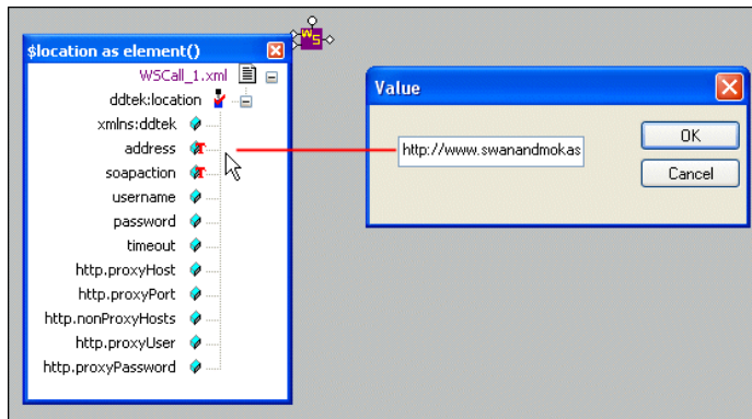
Figure 346. Value for wscall location
