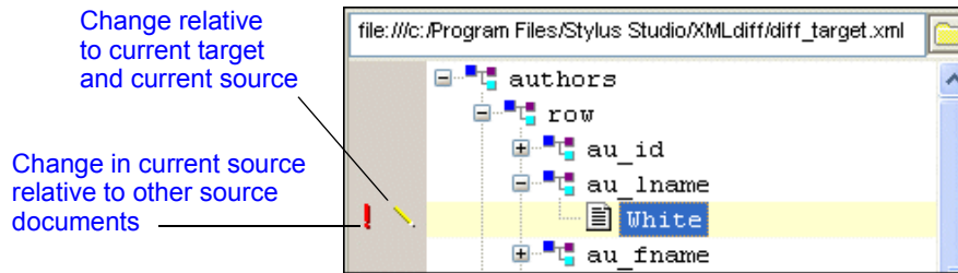
Figure 137. Example of Symbols Used When Diffing Multiple Documents
