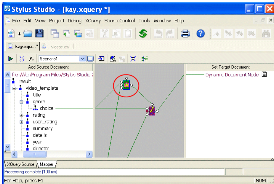
Figure 291. Simple FLWOR Shown in XQuery Mapper
