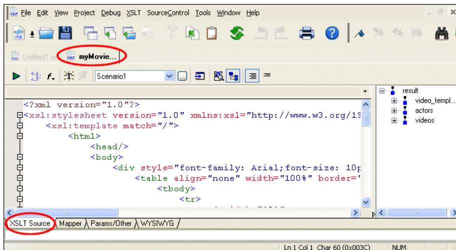
Figure 496. XSLT Generated from the XML Publisher Report
