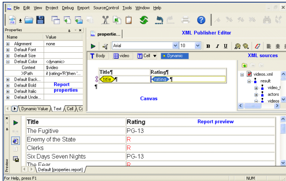
Figure 431. XML Publisher and Report Preview
