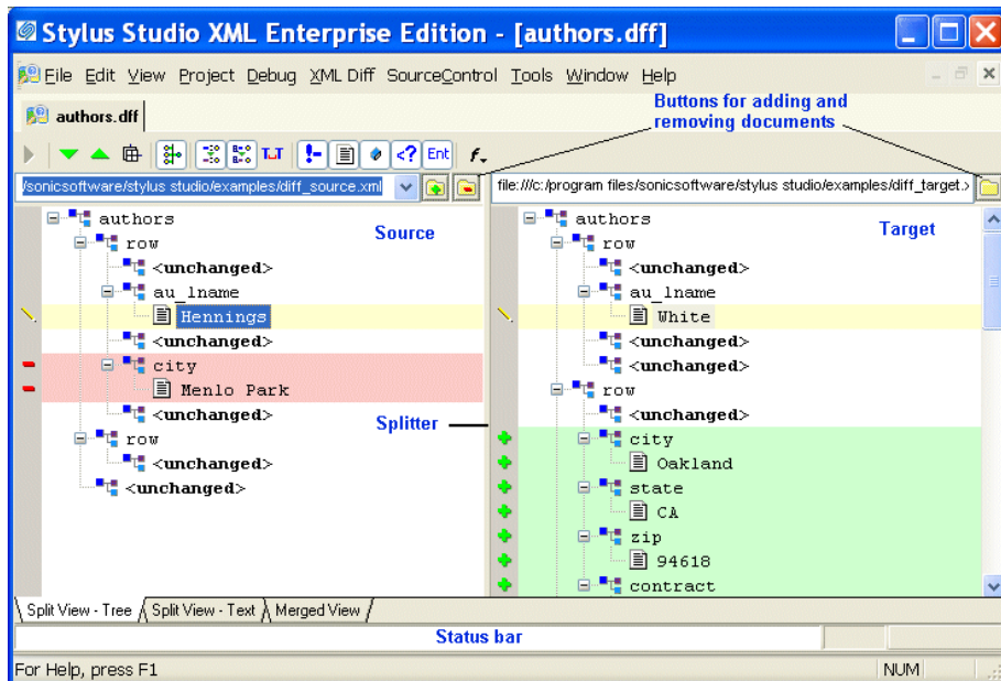
Figure 131. XML Diff Viewer – Split View - Tree
