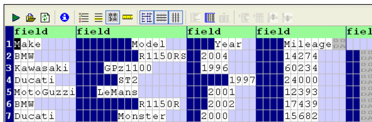
Figure 161. Fields are Aligned by Default
