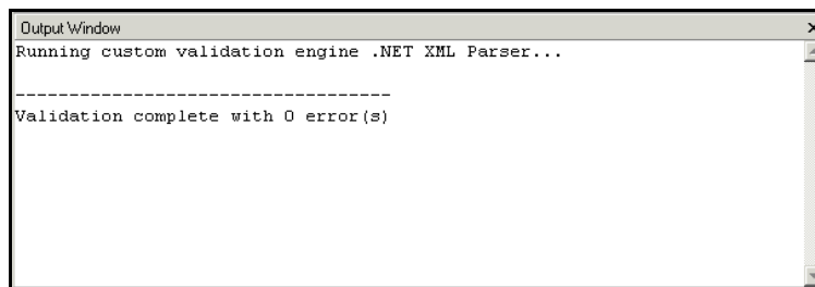
Figure 502. Output Window
