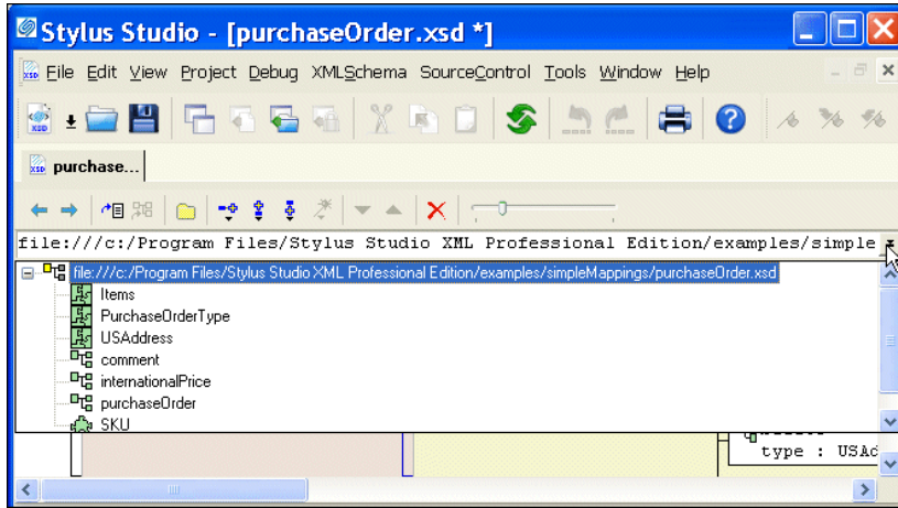
Figure 58. Definition Browser
