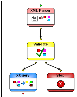
Figure 421. Example XML Parser Node Implementation
