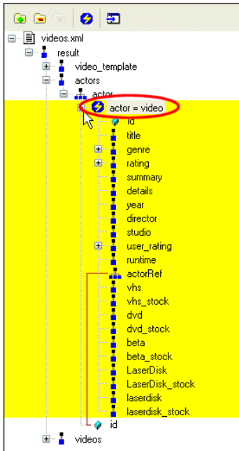
Figure 445. Join Displayed as a Data Source
