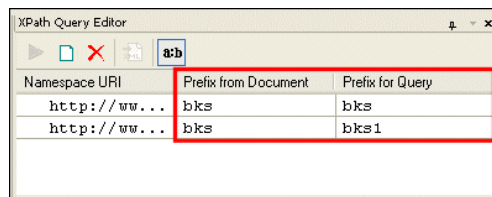
Figure 281. Namespaces Pane
