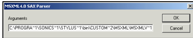
Figure 505. Argument Prompt
