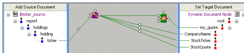
Figure 355. Finished Mapping
