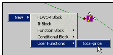
Figure 308. User-Defined Functions
