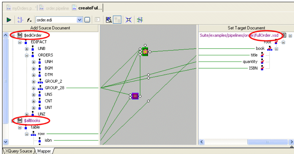
Figure 397. XQuery Mapper Used to Generate createFullOrder.xquery
