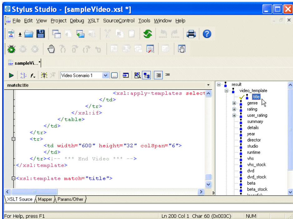
Figure 189. Tree View Lets You Easily Edit XSLT
