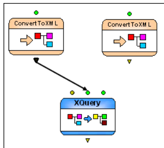
Figure 399. The XML Pipeline’s First Pipe
