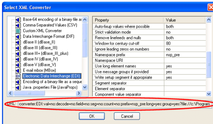
Figure 418. Select XML Converter Dialog Box
