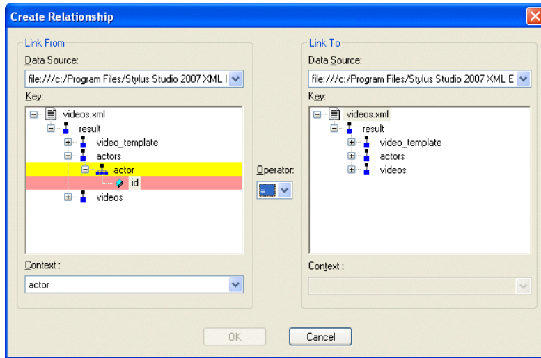
Figure 447. Create Relationship Dialog Box
