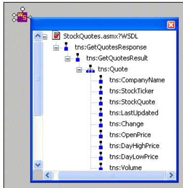
Figure 348. wscall Output Port
