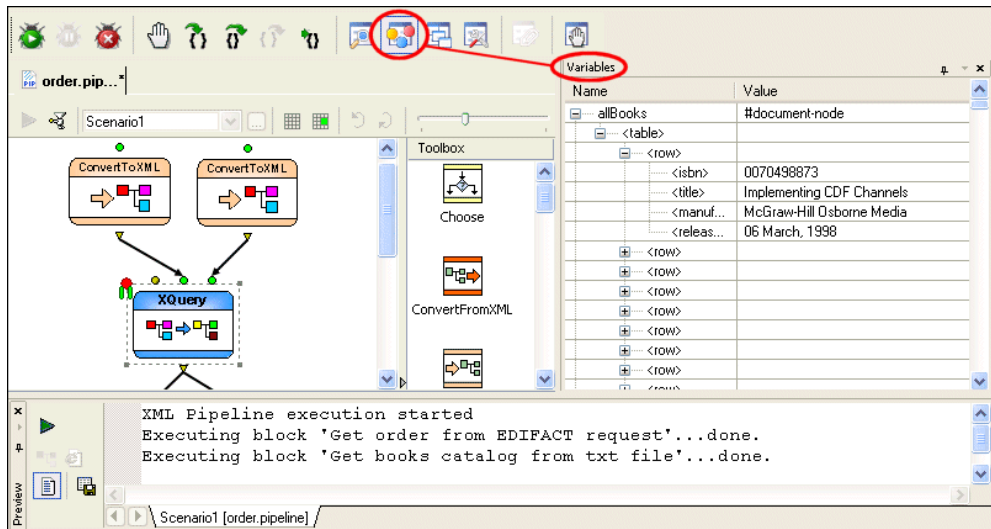
Figure 426. Debugging an XQuery Node in order.pipeline
