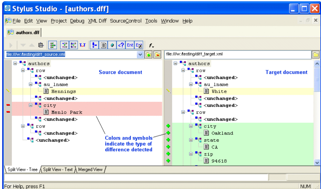
Figure 125. Example of Dified Documents in the XML Diff Viewer
