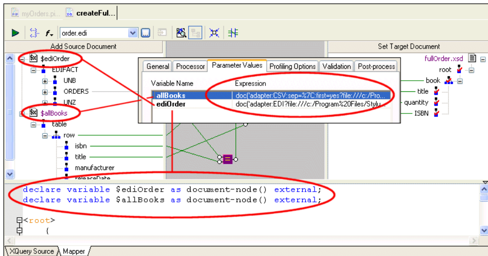
Figure 394. Variables Created for Non-XML Data Sources
