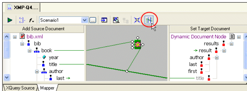
Figure 303. Simply the Mapper by Hiding Links
