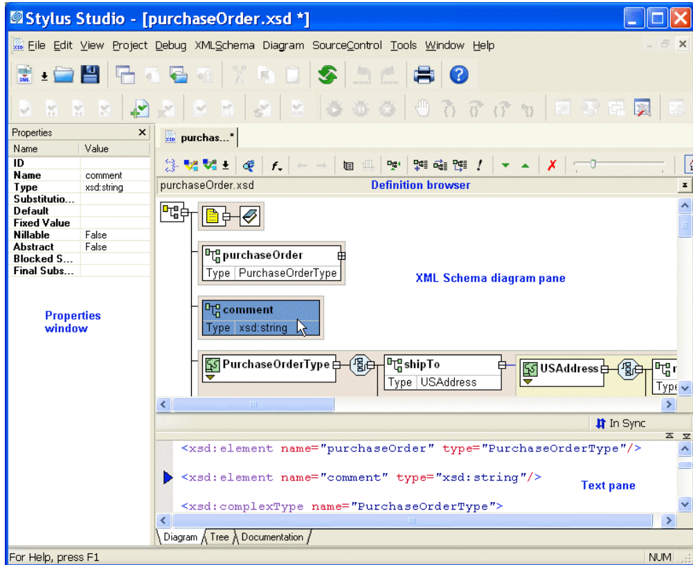
Figure 49. Diagram Tab of the XML Schema Editor
