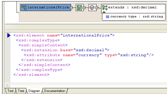
Figure 263. internationalPrice Element in purchaseOrder.xsd
