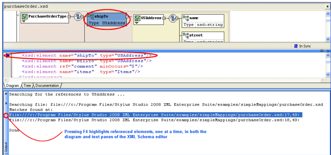
Figure 254. Results of a Search for Referencing Nodes
