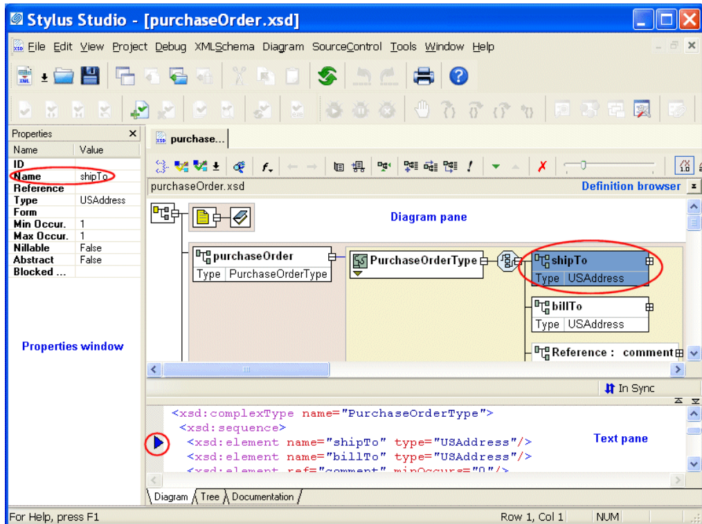
Figure 249. XML Schema Editor Diagram Tab
