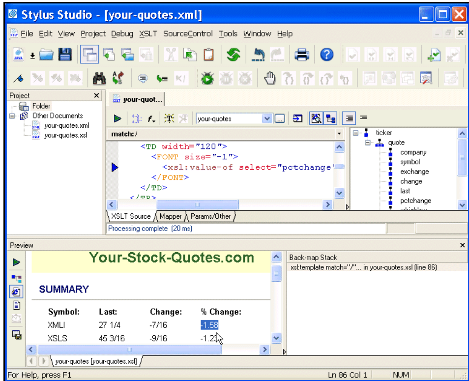
Figure 26. Back-mapping Shows which XSLT Generated a Result
