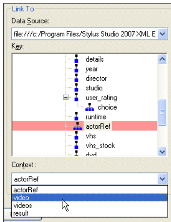
Figure 448. Changing the Context of the Target Node
