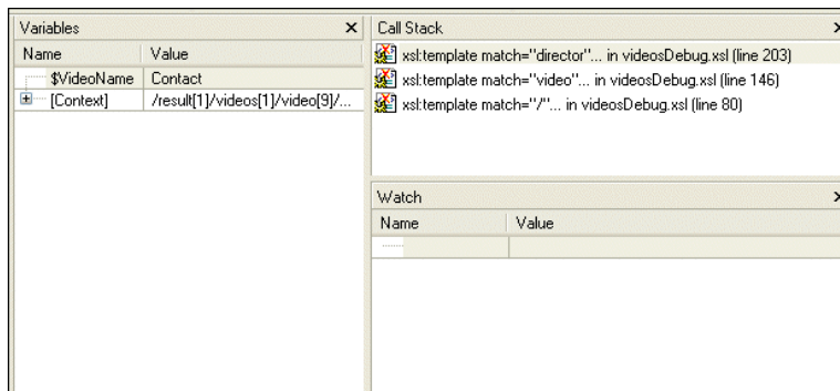
Figure 37. Variable, Call Stack, and Watch Windows Appear During Debugging
