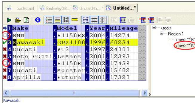
Figure 176. Gray Squares Identify Rows That Match Other Patterns
