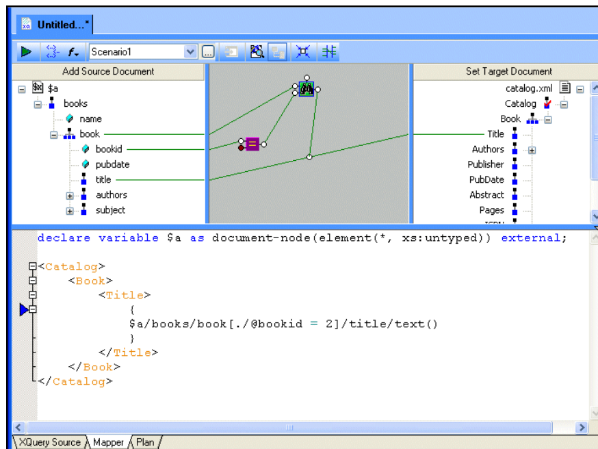
Figure 315. Predicate Block Defined in XQuery Mapper
