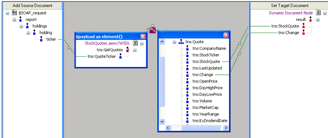
Figure 350. Mapping a wscall Function Block
