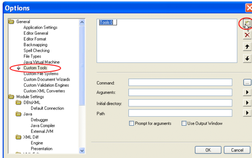
Figure 95. Defining a Custom Tool
