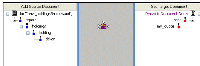
Figure 351. Adding Source and Target Documents
