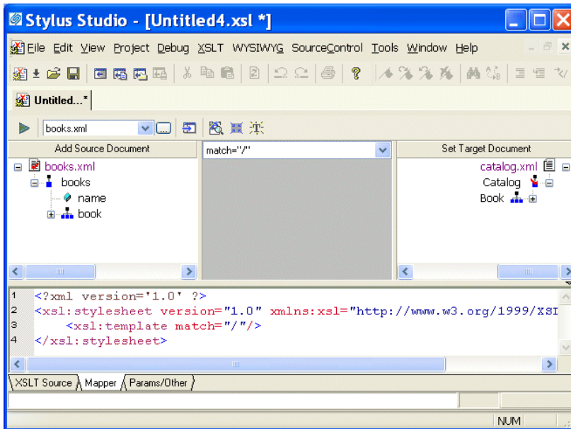
Figure 29. XSLT Mapper Tab with Source and Target Documents
