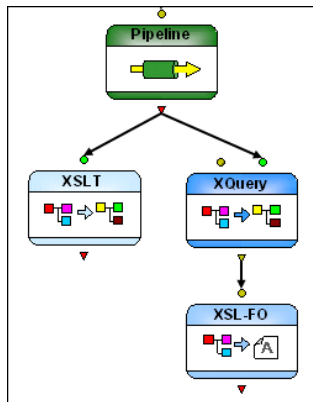
Figure 410. XQuery and XSLT Nodes in getHoldings.pipeline
