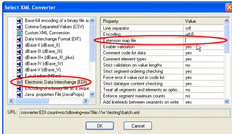
Figure 184. Specifying a Custom EDI Message Type
