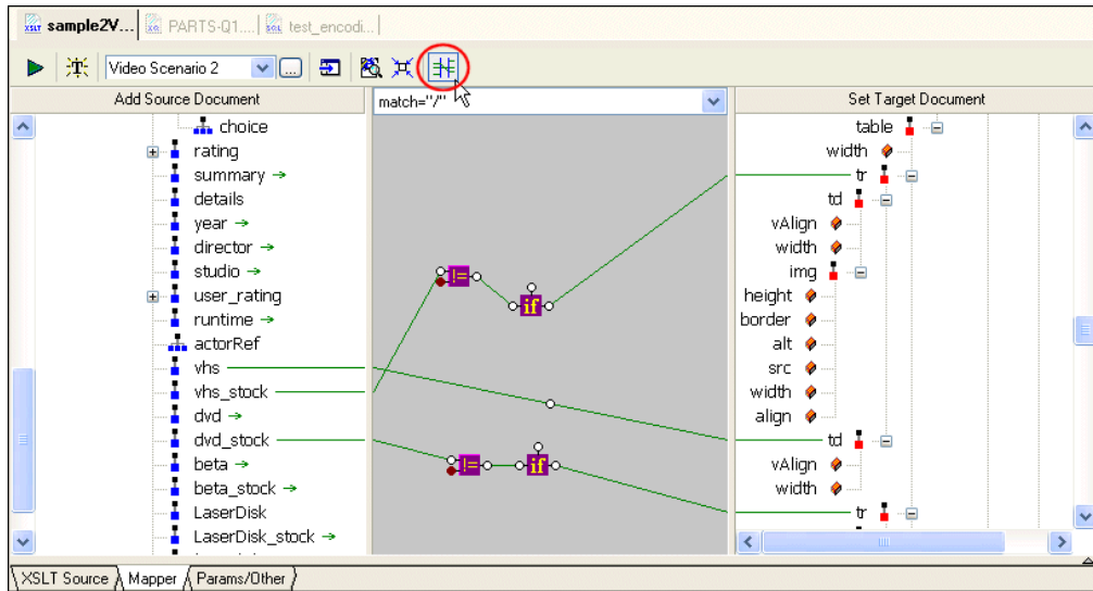
Figure 216. Simply the Mapper by Hiding Links
