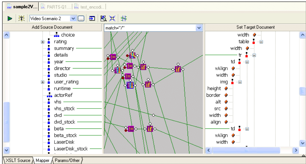
Figure 215. Mapper Shows Links to All Nodes, Visible or Not
