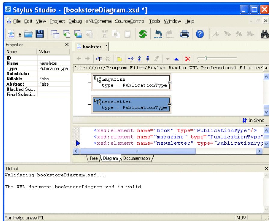
Figure 72. Validation of bookstoreDiagram.xsd
