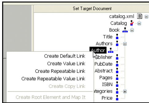
Figure 224. Shortcut Menu for Target Document Operations
