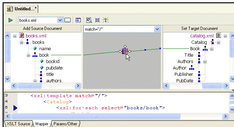
Figure 30. xs1:for-each Block Displayed by the XSLT Mapper
