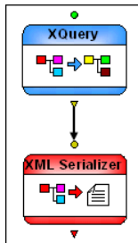
Figure 422. Example XML Serializer Node Implementation
