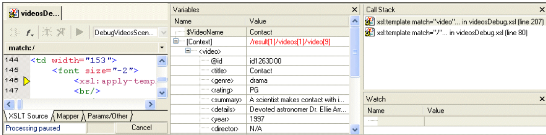
Figure 40. Stepping Out Advances the Processor
