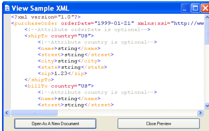
Figure 252. Sample of XML Based on XML Schema
