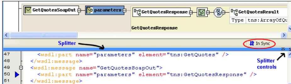
Figure 374. Diagram and Text Panes in the WSDL Editor
