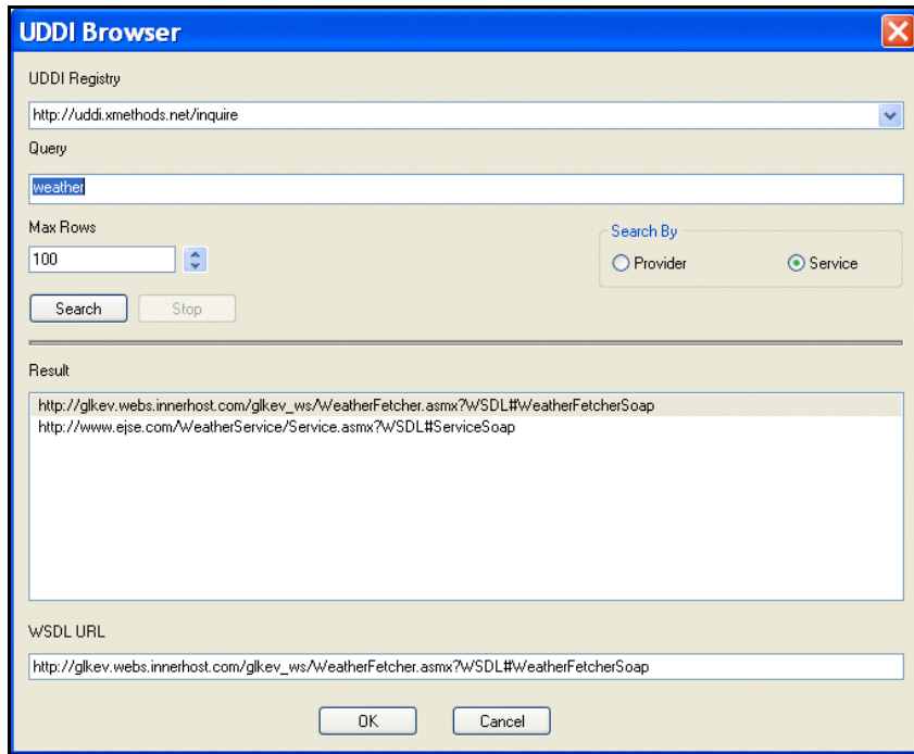
Figure 364. UDDI Browser result
