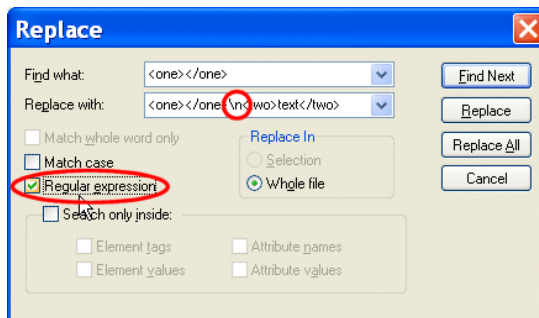
Figure 107. Replacing Text Using Regular Expressions
